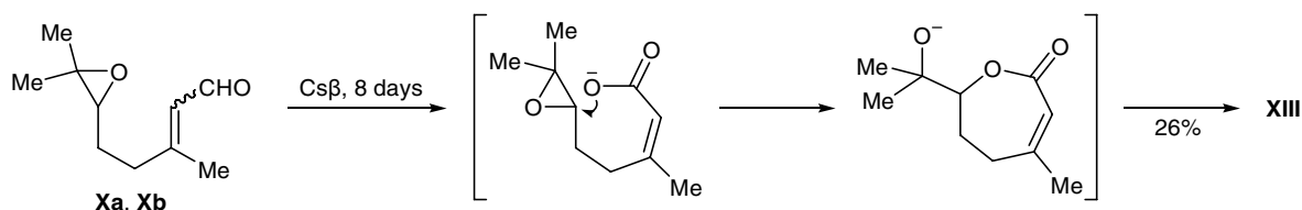
Scheme 4.
